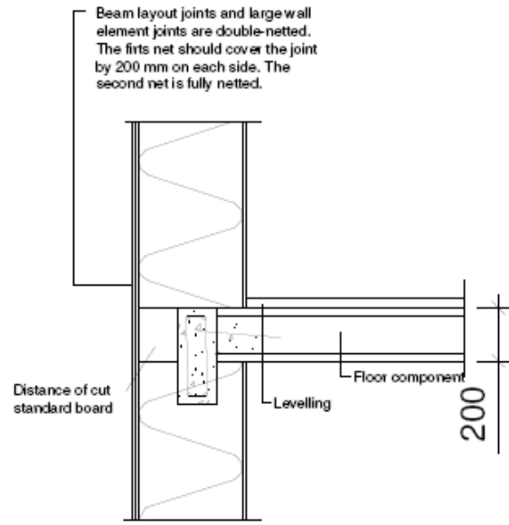
Detail: Fastening of concrete floor structure
