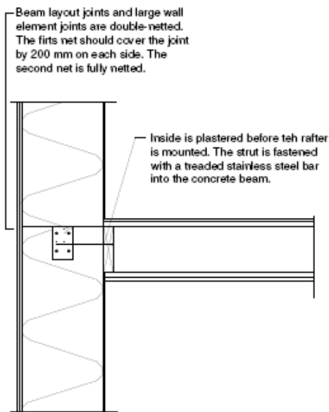
Detail: Fastening of wooden floor structure
